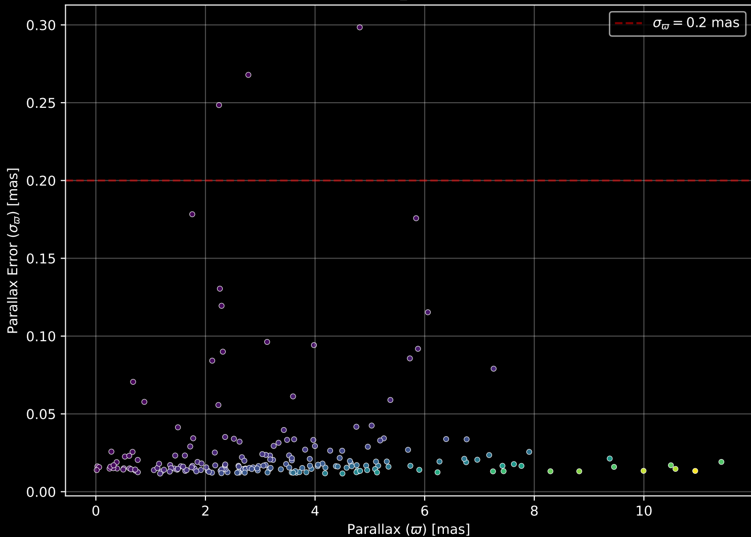
APOGEE DR17 Field: [165+61_MGA] Parallax Quality (n= 196)
