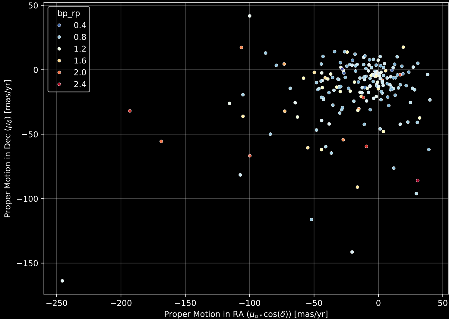
APOGEE DR17 Field: [165+61_MGA] Proper Motion Diagram (n= 196)
