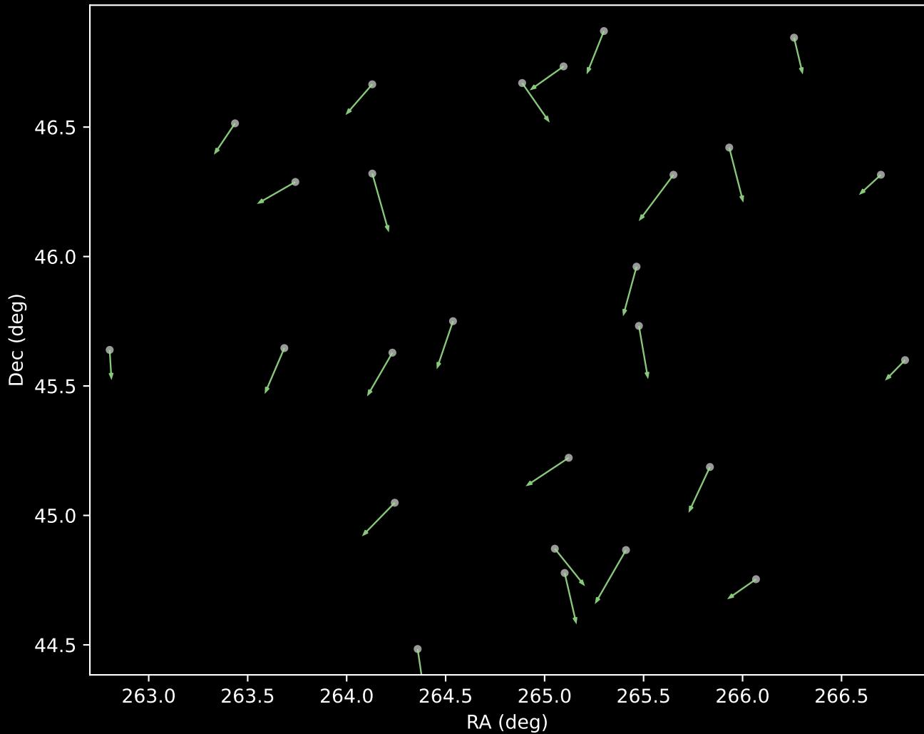
APOGEE DR17 Cluster 5 Proper Motion Vectors (n=26)
