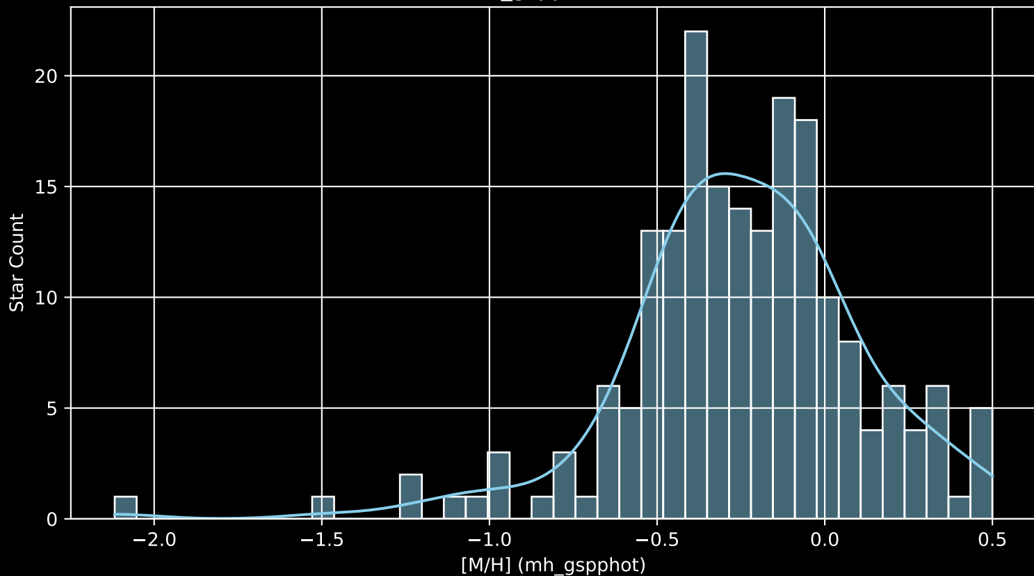
APOGEE DR17 Field: [165+61_MGA [M/H] (mh_gspphot) (n= 196)
