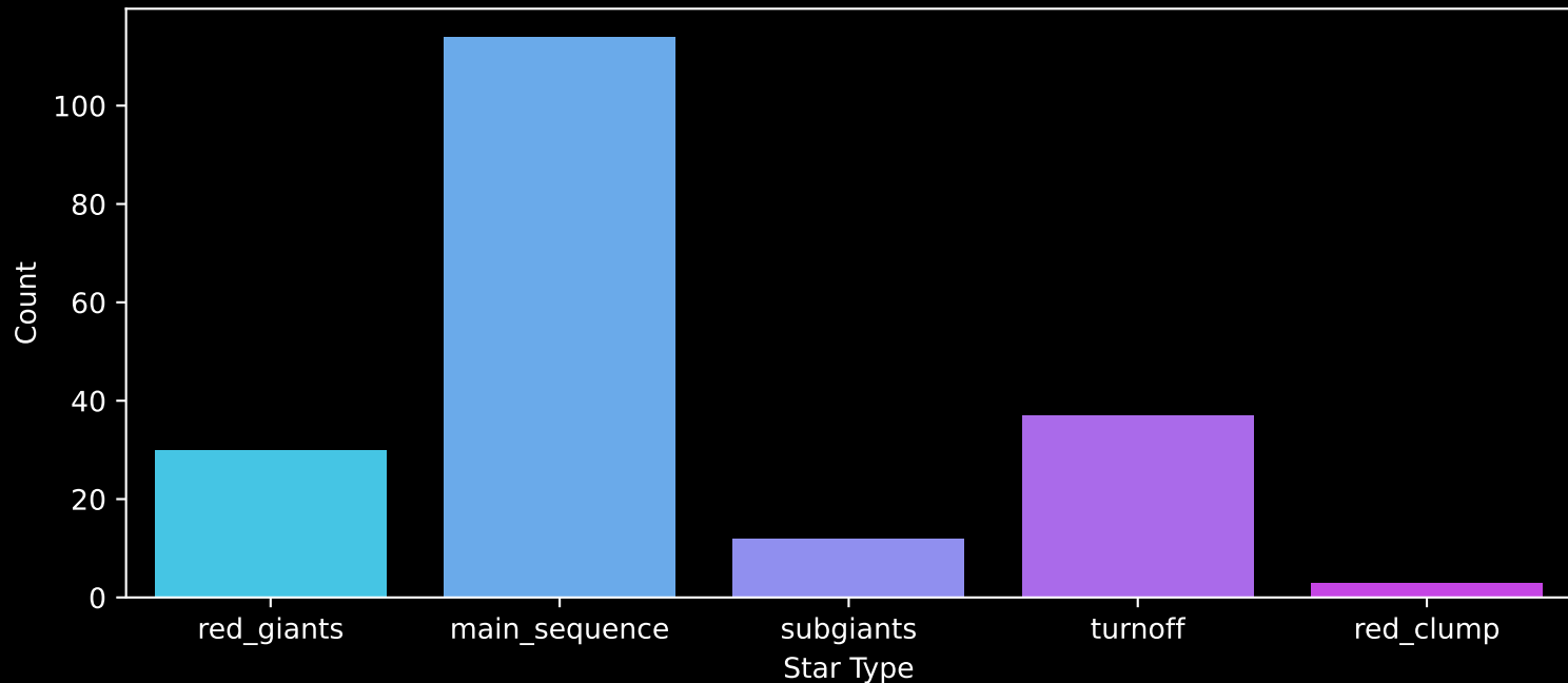
APOGEE DR17 Field: [165+61_MGA] Count plot of Star Type
