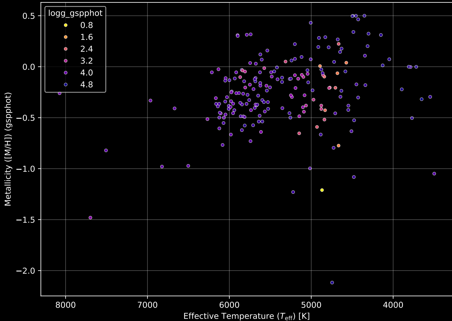
APOGEE DR17 Field: [165+61_MGA] Stellar Population Parameters (n= 196)
