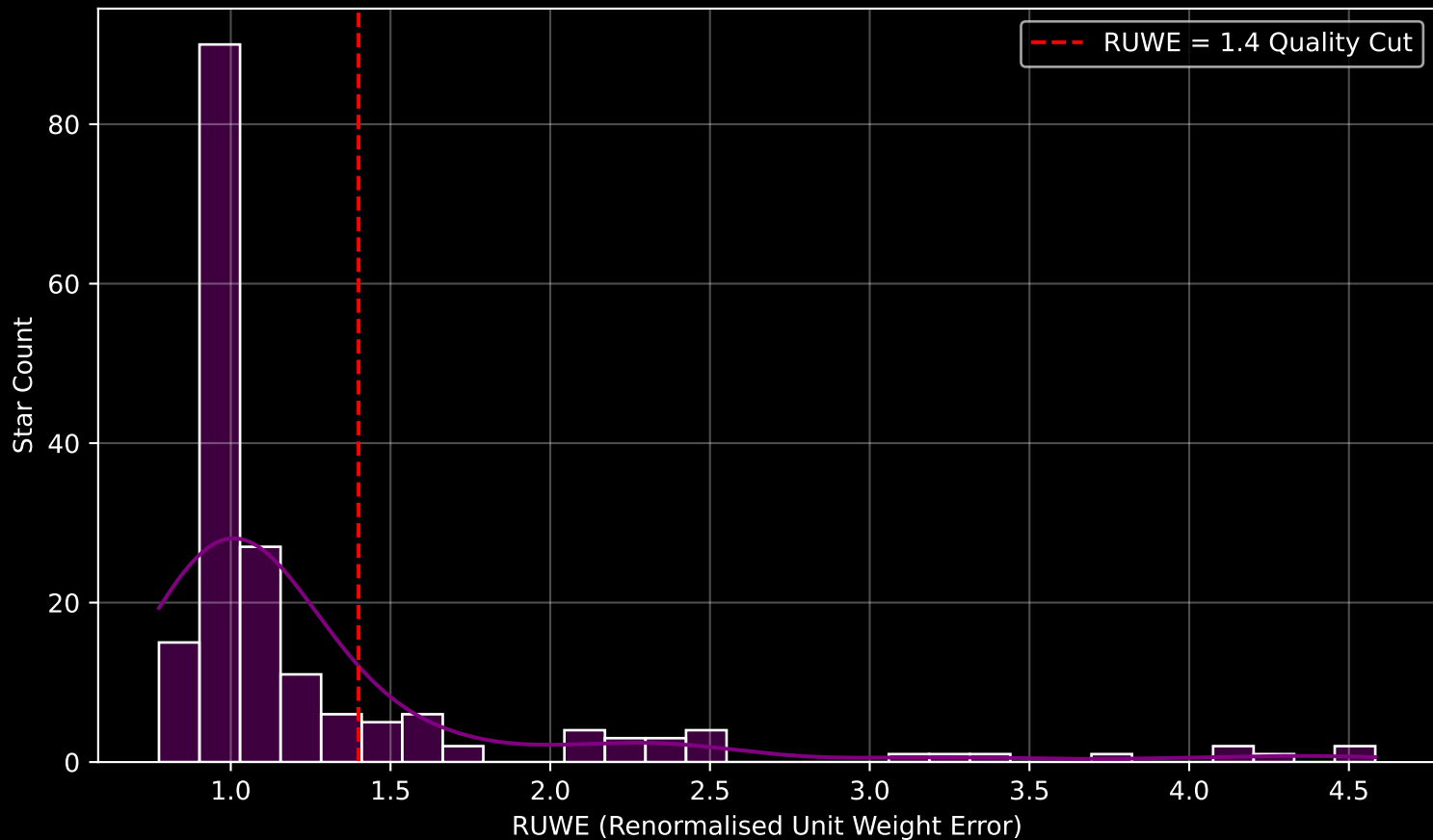
GAPOGEE DR17 Field [165+61_MGA] RUWE Distribution (n= 185)
